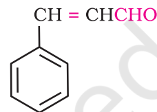
Cinnamaldehyde
