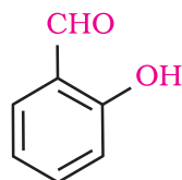
Salicylaldehyde
