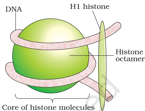
Figure 5.4a Nucleosome
