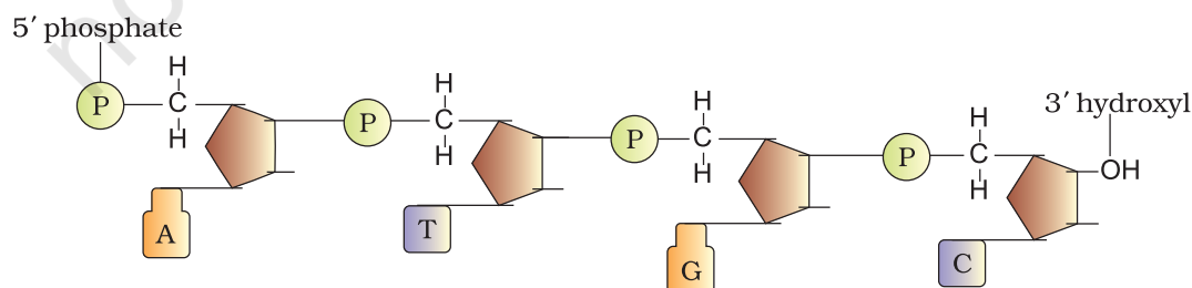
Figure 5.1 A Polynucleotide chain
