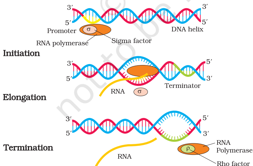
Figure 5.10 Process of Transcription in Bacteria
