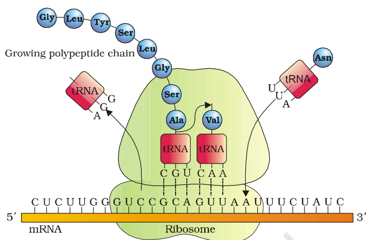
Figure 5.13 Translation
