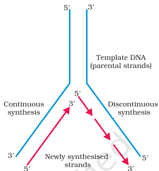
Figure 5.8 Replicating Fork
