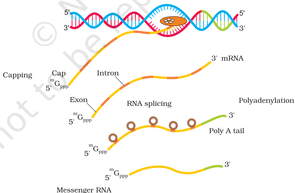
Figure 5.11 Process of Transcription in Eukaryotes
