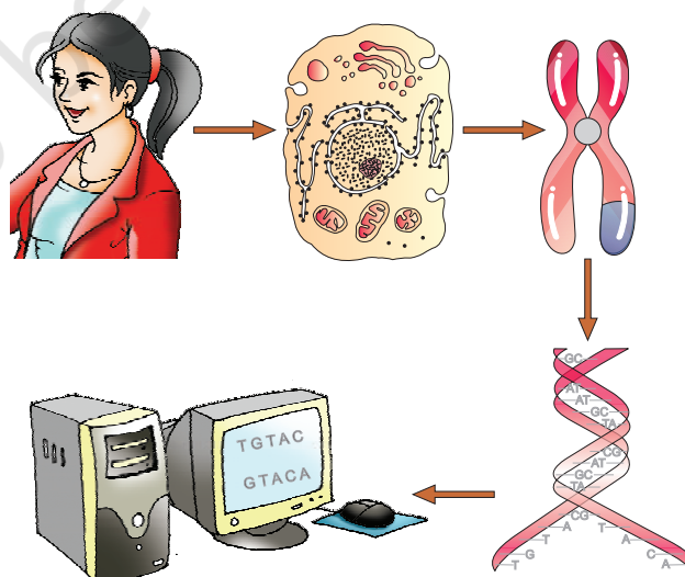
Figure 5.15 A representative diagram of human genome project
