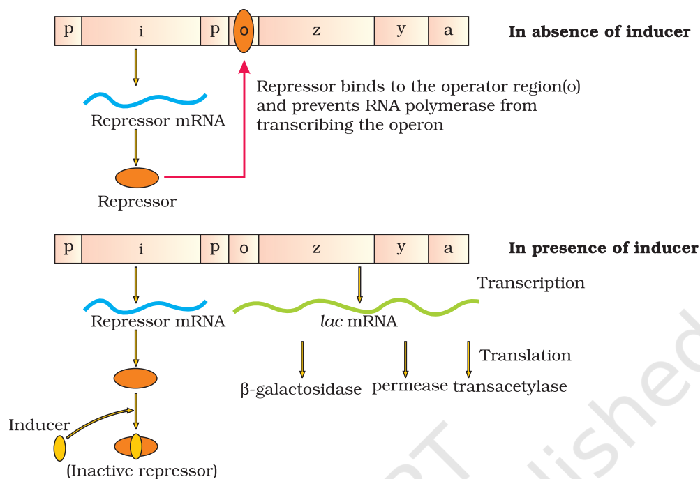
Figure 5.14 The lac Operon
