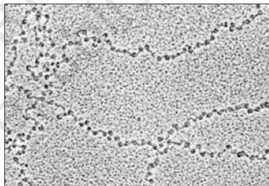
Figure 5.4b EM picture - 'Beads-on-String'
