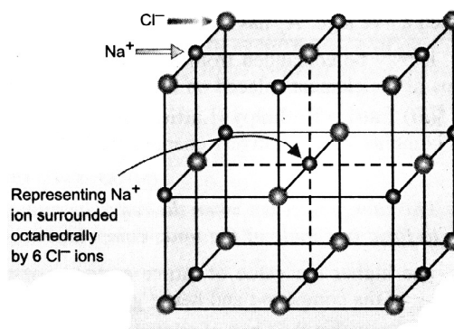
Crystal structure of NaCl
