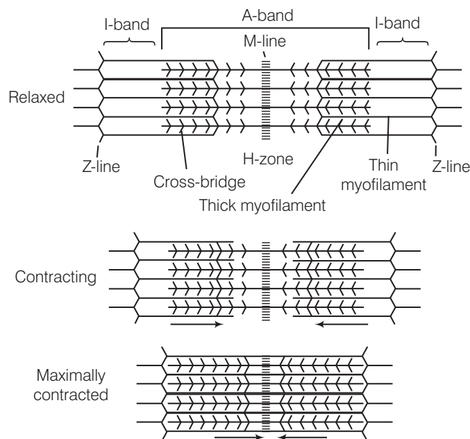
Sliding filament theory of muscle contraction
