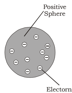
Thomson's proposed model of atom.
