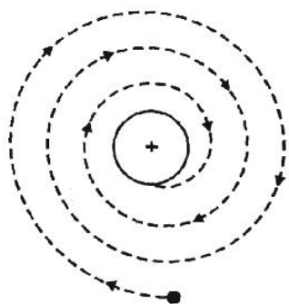
ELECTRON FALLING INTO THE NUCLEUS
