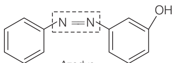
Azodye
