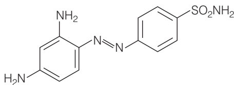
Prontosil
