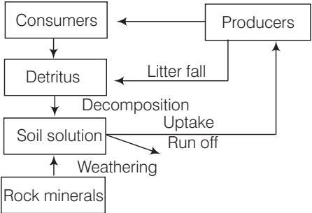
A simplified model of phosphorus cycling in a terrestrial ecosystem
