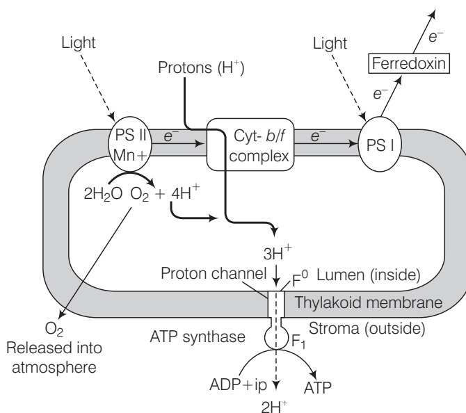
Proton ( H^+ ) gradient and ATP formation
