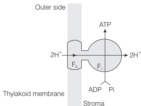
Diagrammatic presentation of ATP synthesis in chloroplast
