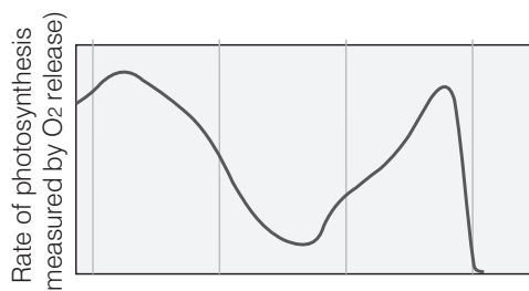
Graph showing action spectrum of photosynthesis
