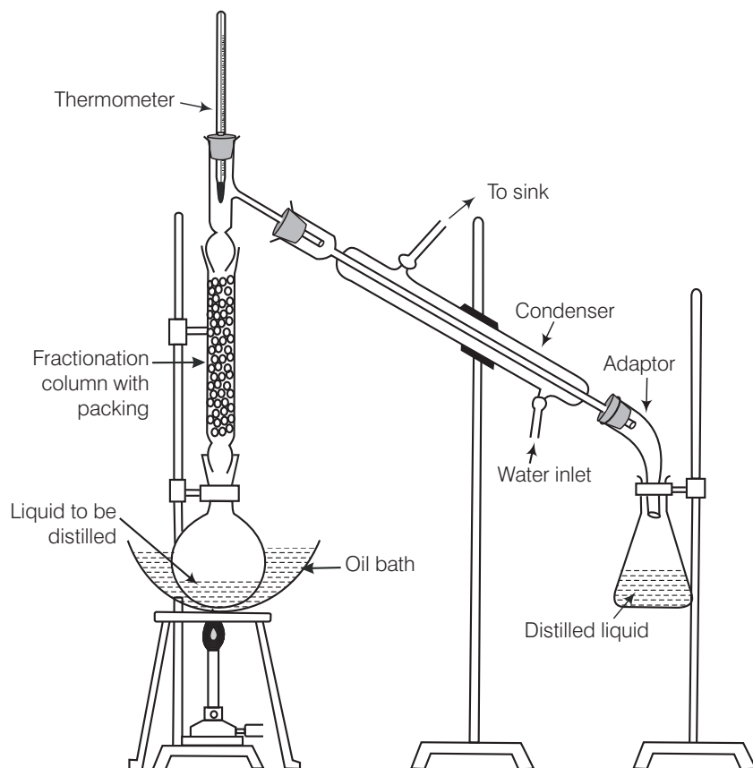
Fractional distillation
