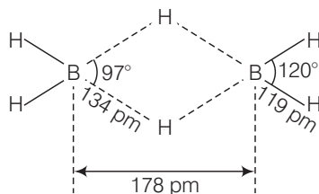
Structure of diborane
