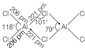
Dimer structure of \text{AlCl}_3 (\text{Al}_2\text{Cl}_6)
