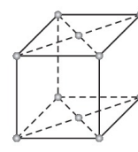
End centred
