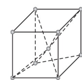
Body centred
