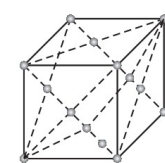
Face centred
