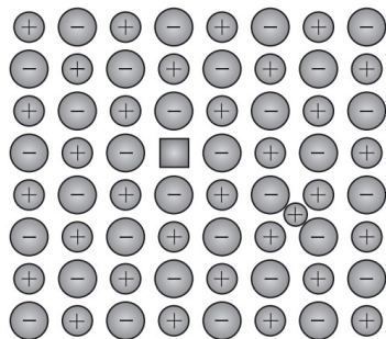
Frenkel defects
