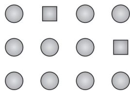
Vacancy defects
