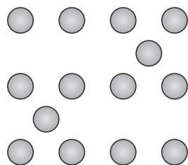
Interstitial defects
