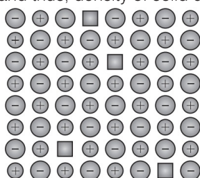
Schottky defects
